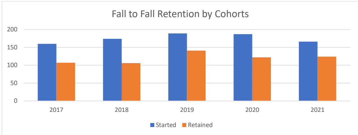
Figure 1. Retention
