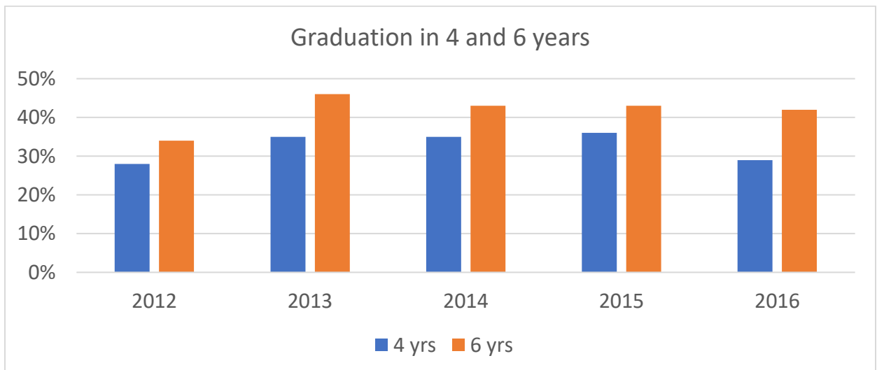
Figure 2. Graduation Rates
